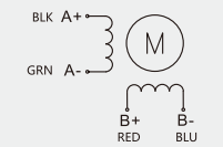
Connection of 4-wire motor
