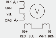
Series connection of 8-wire motor
