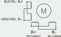
Parallel connection of 8-wire motor
