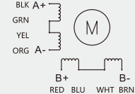
Series connection of 8-wire motor
